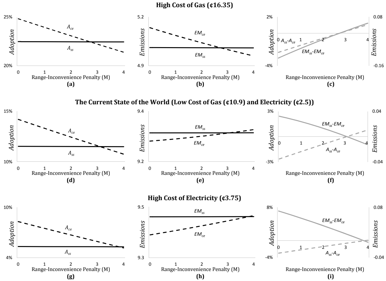
FIGURE 5.2. The Impact of Energy Cost Evolution on Adoption and Emissions
