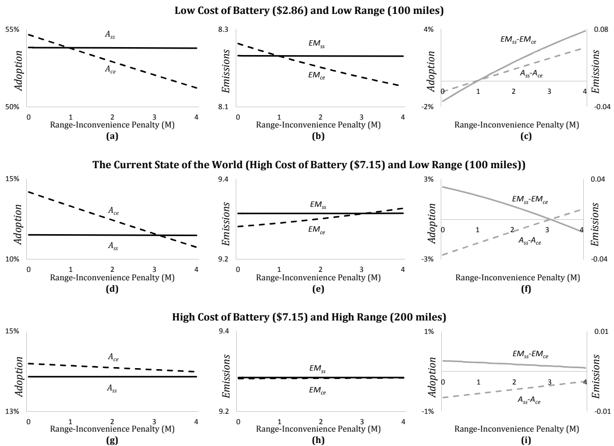
FIGURE 5.1. The Impact of Technological Evolution on Adoption and Emissions
